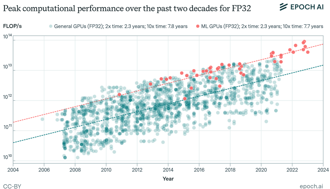
Figure 52: Currently observed trends in the efficiency of hardware used for ML over the last decades. We can see a clear year by year increase in peak computational performance (Hobbahn et al., 2023).
