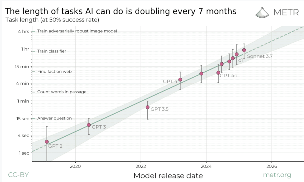
Figure 32: The image shows a result from METR which measured the task length horizon on specific software engineering tasks (Kwa et al., 2025).
