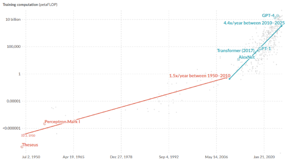
Figure 36: Exponential growth of computation in the training of notable AI systems. Computation is measured in total peta FLOP, which is 10e15 floating-point operations (Giattino et al., 2023). (interactive version on website)
