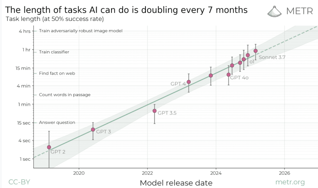
Figure 32: The image shows a result from METR which measured the task length horizon on specific software engineering tasks (Kwa et al., 2025).
