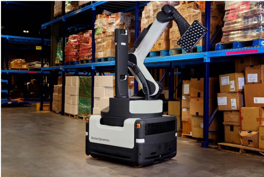
Figure 20: Boston Dynamics' Stretch robot that can autonomously unload shipping containers, lift up to 50 pounds, and clear away missed boxes along the way ( Boston Dynamics, 2024 ).
