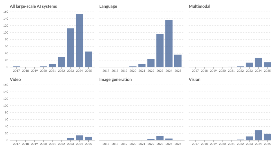
Figure 22: Number of large-scale AI systems released per year. Describes the specific area, application, or field in which a large-scale AI model is designed to operate. The 2025 data is incomplete and was last updated 01 June 2025 ( Giattino et al., 2023 ). (interactive version on website)
