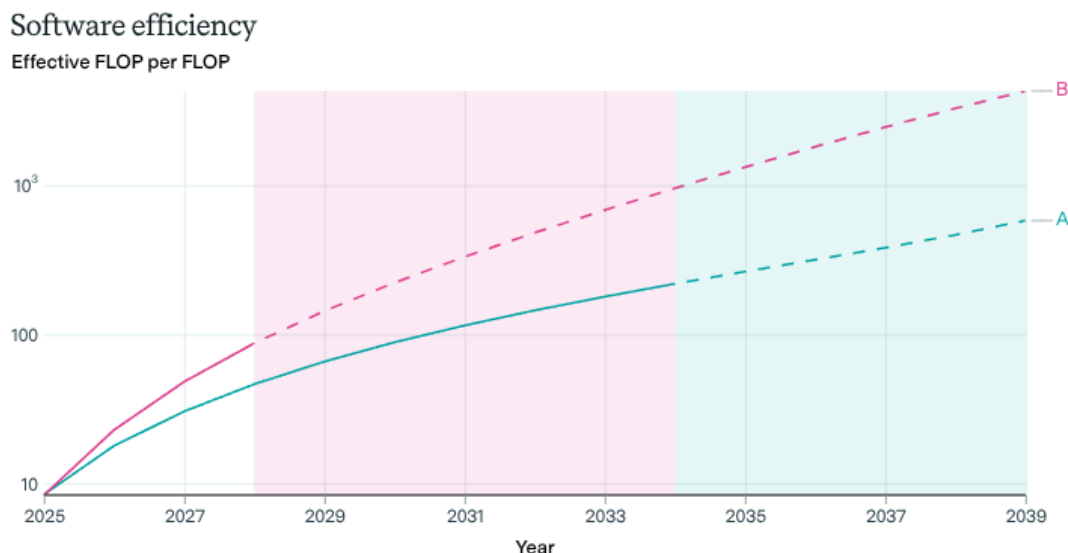
Figure 55: A forecast of the future using the Growth and AI Transition Endogenous (GATE) playground. This graph shows algorithmic improvements over time. By developing better algorithms and using higher-quality data, it becomes possible to do more with the same hardware (measured in units of “effective FLOP per FLOP”). The red line showcases aggressive parameter settings, green is conservative parameter settings. The red zone highlights the difference in timelines to full automation between aggressive and conservative models ( Epoch AI, 2025 ).
