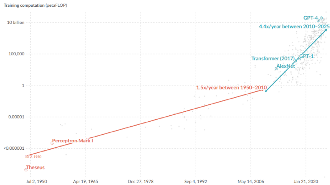
Figure 36: Exponential growth of computation in the training of notable AI systems. Computation is measured in total peta FLOP, which is 10^{15} floating-point operations (Giattino et al., 2023). (interactive version on website)
