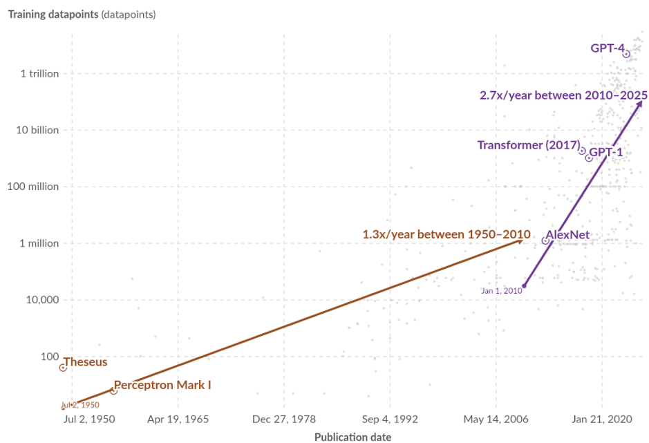
Figure 35: Exponential growth of datapoints used to train notable AI systems. Each domain has a specific data point unit; for example, for vision it is images, for language it is words, and for games it is timesteps. This means systems can only be compared directly within the same domain (Giattino et al., 2023). (interactive version on website)
