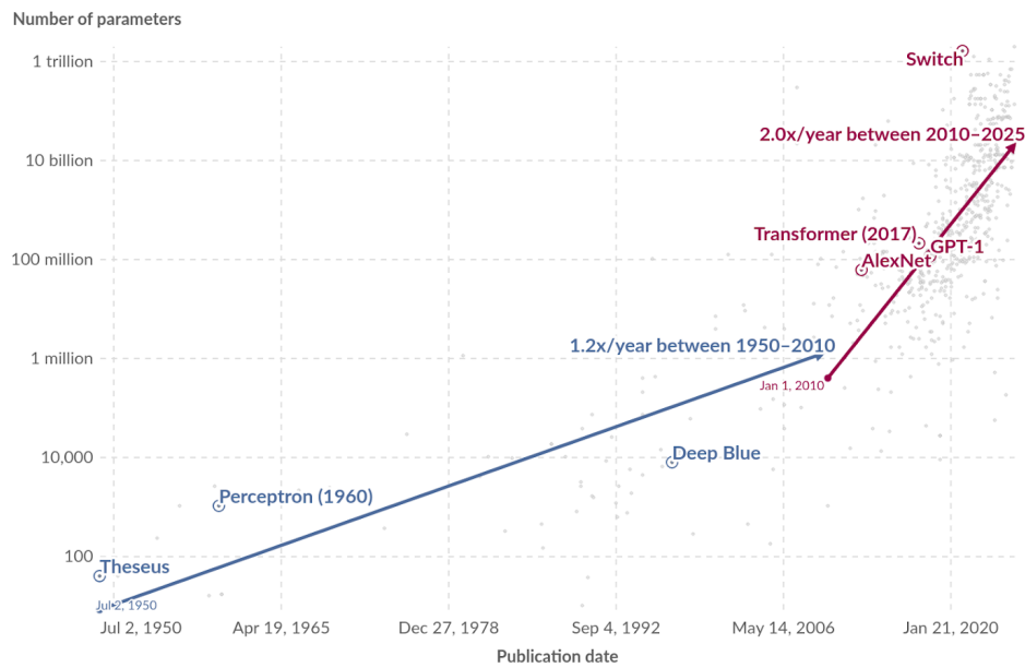
Figure 34: Exponential growth of parameters in notable AI systems. Parameters are variables in an AI system whose values are adjusted during training to establish how input data gets transformed into the desired output; for example, the connection weights in an artificial neural network (Giattino et al., 2023). (interactive version on website)
