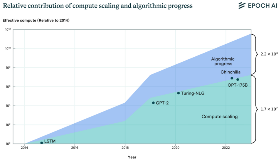
Figure 54: Estimates of the contributions of scaling and algorithmic innovation in terms of the raw compute that would be naively needed to achieve a state-of-the-art level of performance. The contribution of algorithmic progress is roughly half as much as that of compute scaling (Ho et al., 2024)
