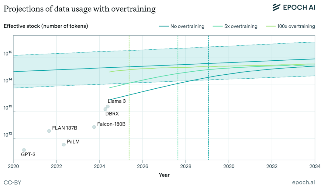
Figure 45: Projections of future dataset sizes according to three different scaling policies. Depending on the degree of overtraining, the stock is fully used between 2025 and 2030 (Villalobos et al., 2024).
