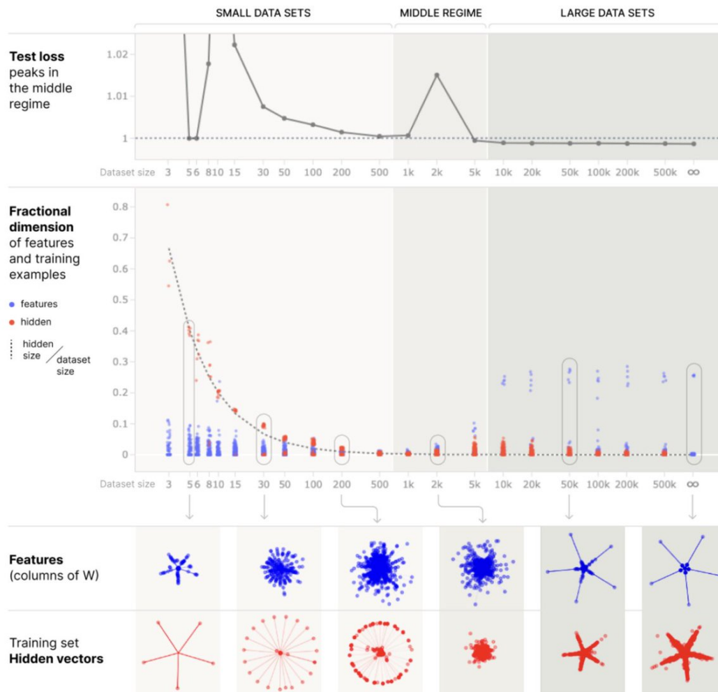
Figure 78: From Superposition, Memorization, and Double Descent (Anthropic, 2023)
