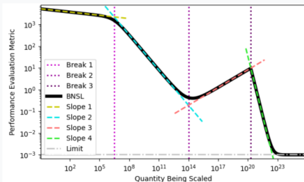
Figure 37: A Broken Neural Scaling Law example (dark black solid line) (with 3 breaks where purple dotted lines intersect with dark black solid line) contains 4 individual power law segments (where the dashed lines that are yellow, blue, red, and green overlap with the dark black solid line). The 1st and 2nd break are very smooth; the 3rd break is very sharp (Caballero et al., 2023).
