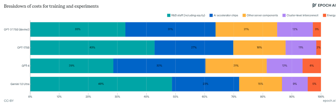
Figure 60: Breakdown of model development costs for selected models. Hardware costs are amortized to the total number of chip-hours spent on experiments and training. R&D staff costs cover the duration of development, from initial experiments to publication (Cottier et al., 2025).
