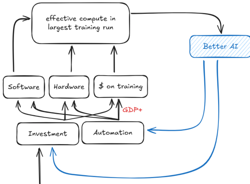
Figure 50: A summary of What a Compute-Centric Framework Says About Takeoff Speeds (Davidson, 2024)
