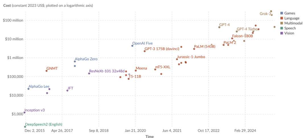
Figure 61: Hardware and energy cost to train notable AI systems. This data is expressed in US dollars, adjusted for inflation (Our World in Data, 2023). (interactive version on website)
