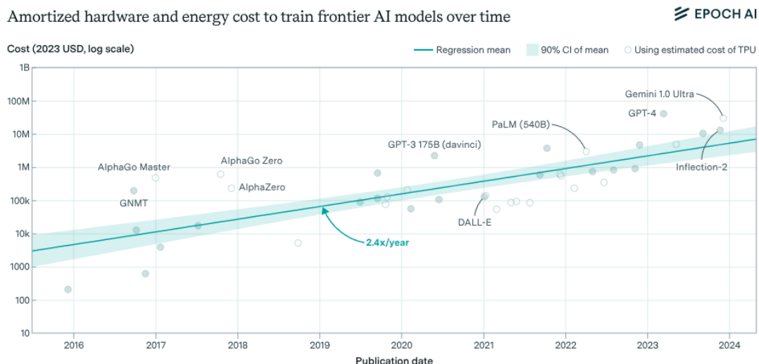
Figure 59: Amortized hardware cost plus energy cost for the final training run of frontier models. The selected models are among the top 10 most compute-intensive for their time. Amortized hardware costs are the product of training chip-hours and a depreciated hardware cost, with 23% overhead added for cluster-level networking. Open circles indicate costs which used an estimated production cost of Google TPU hardware. These costs are generally more uncertain than the others, which used actual price data rather than estimates (Cottier et al., 2025).
