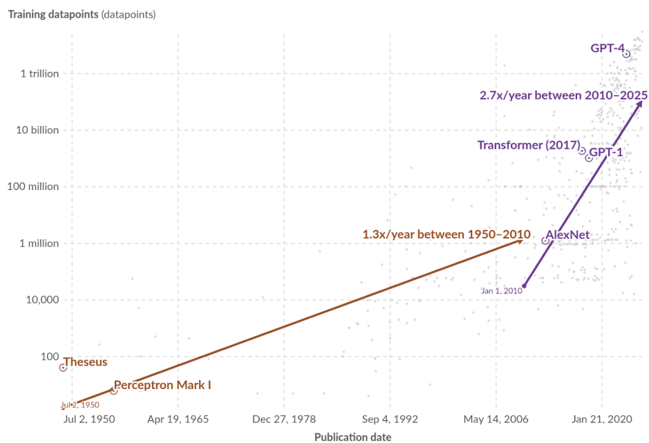
Figure 32: Exponential growth of datapoints used to train notable AI systems. Each domain has a specific data point unit; for example, for vision it is images, for language it is words, and for games it is timesteps. This means systems can only be compared directly within the same domain (Giattino et al., 2023). (interactive version on website)
