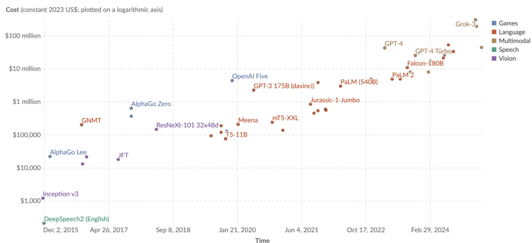
Figure 58: Hardware and energy cost to train notable AI systems. This data is expressed in US dollars, adjusted for inflation (Our World in Data, 2023). (interactive version on website)
