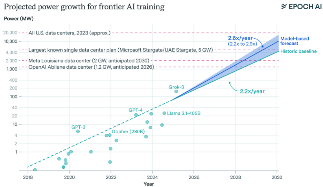
Figure 63: Historic trend and forecast for the electricity demand of the largest individual frontier training runs (You et al., 2025).
