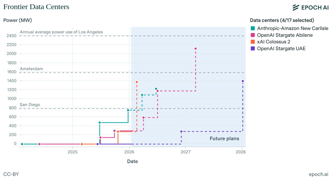
Figure 64: The projected power consumption for planned frontier datacenters for selected AI companies (Epoch AI, 2025).
