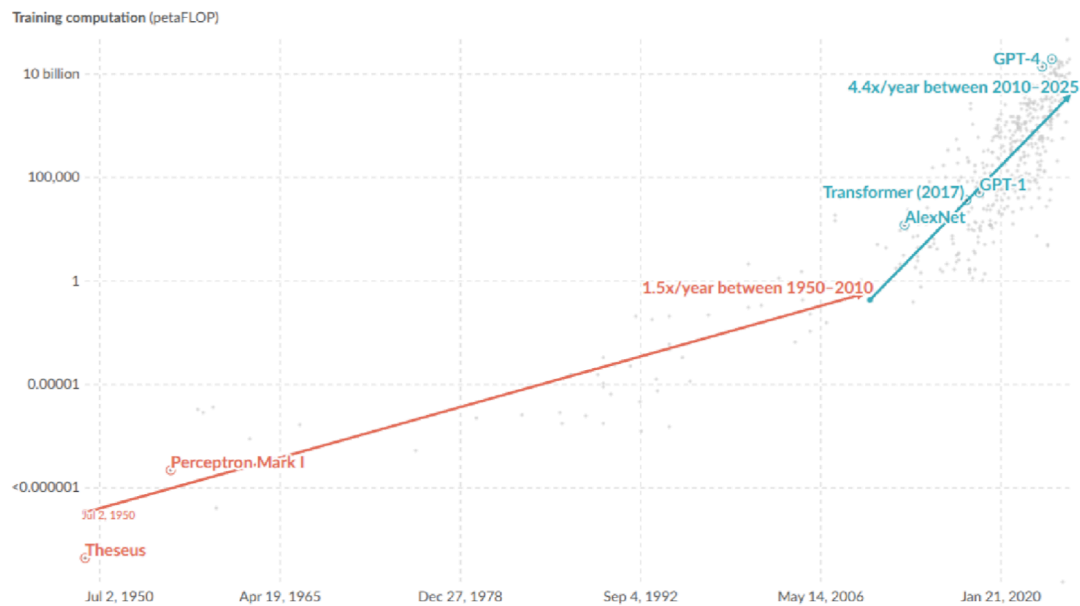
Figure 33: Exponential growth of computation in the training of notable AI systems. Computation is measured in total peta FLOP, which is 10^{15} floating-point operations (Giattino et al., 2023). (interactive version on website)
