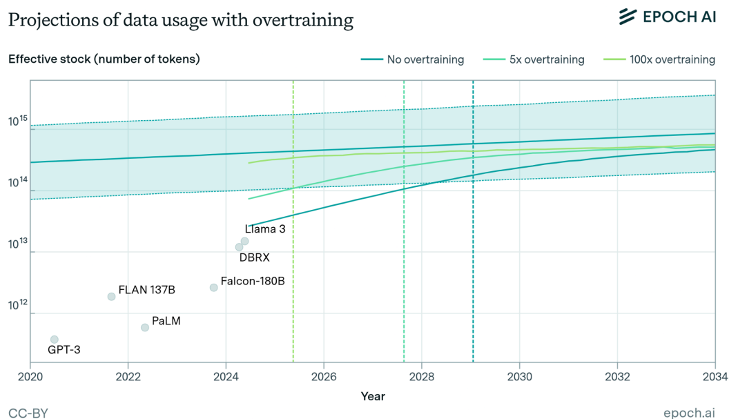
Figure 42: Projections of future dataset sizes according to three different scaling policies. Depending on the degree of overtraining, the stock is fully used between 2025 and 2030 (Villalobos et al., 2024).
