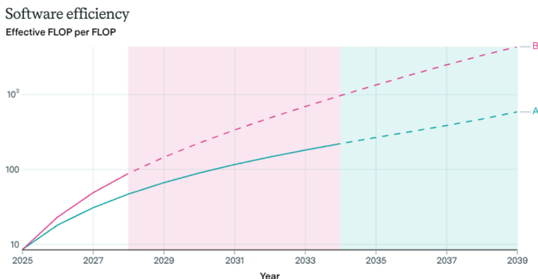
Figure 52: A forecast of the future using the Growth and AI Transition Endogenous (GATE) playground. This graph shows algorithmic improvements over time. By developing better algorithms and using higher-quality data, it becomes possible to do more with the same hardware (measured in units of “effective FLOP per FLOP”). The red line showcases aggressive parameter settings, green is conservative parameter settings. The red zone highlights the difference in timelines to full automation between aggressive and conservative models ( Epoch AI, 2025 ).
