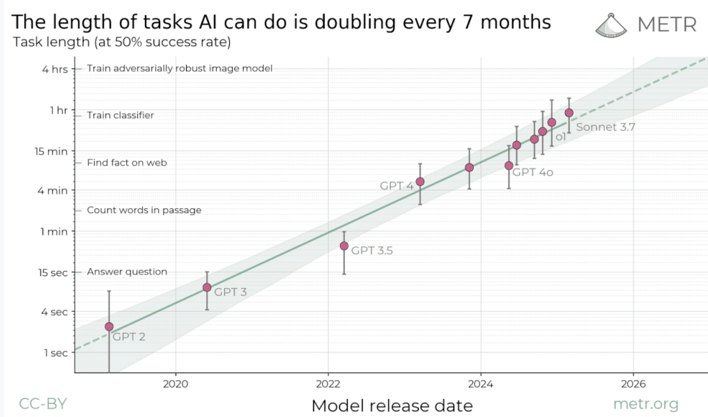
Figure 29: The image shows a result from METR which measured the task length horizon on specific software engineering tasks (Kwa et al., 2025).
