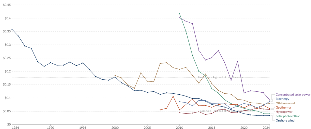
Figure 66: The levelized cost of energy (LCOE) accounts for everything, the cost of building the power plant, plus the ongoing costs in keeping it operational over the lifetime of the plant. The cost of energy generation per watt has been falling for decades, and even more dramatically for renewable sources ( Our World in Data, 2026 ). (interactive version on website)
