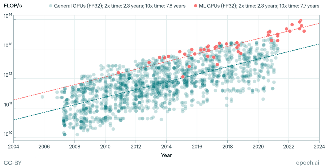
Figure 49: Currently observed trends in the efficiency of hardware used for ML over the last decades. We can see a clear year by year increase in peak computational performance ( Hobbahn et al., 2023 ).
