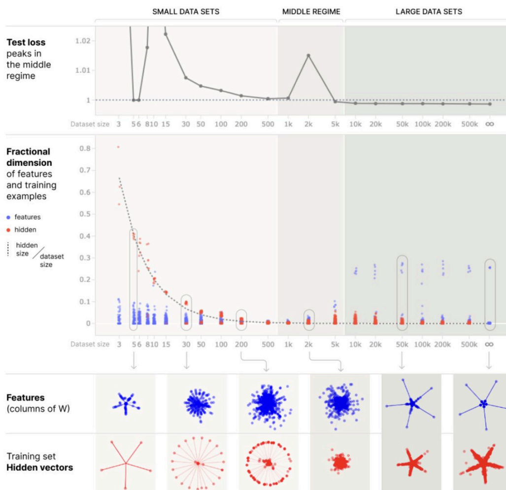
Figure 75: From Superposition, Memorization, and Double Descent ( Anthropic, 2023 )
