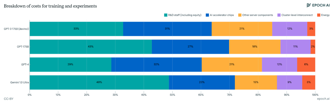
Figure 57: Breakdown of model development costs for selected models. Hardware costs are amortized to the total number of chip-hours spent on experiments and training. R&D staff costs cover the duration of development, from initial experiments to publication (Cottier et al., 2025).
