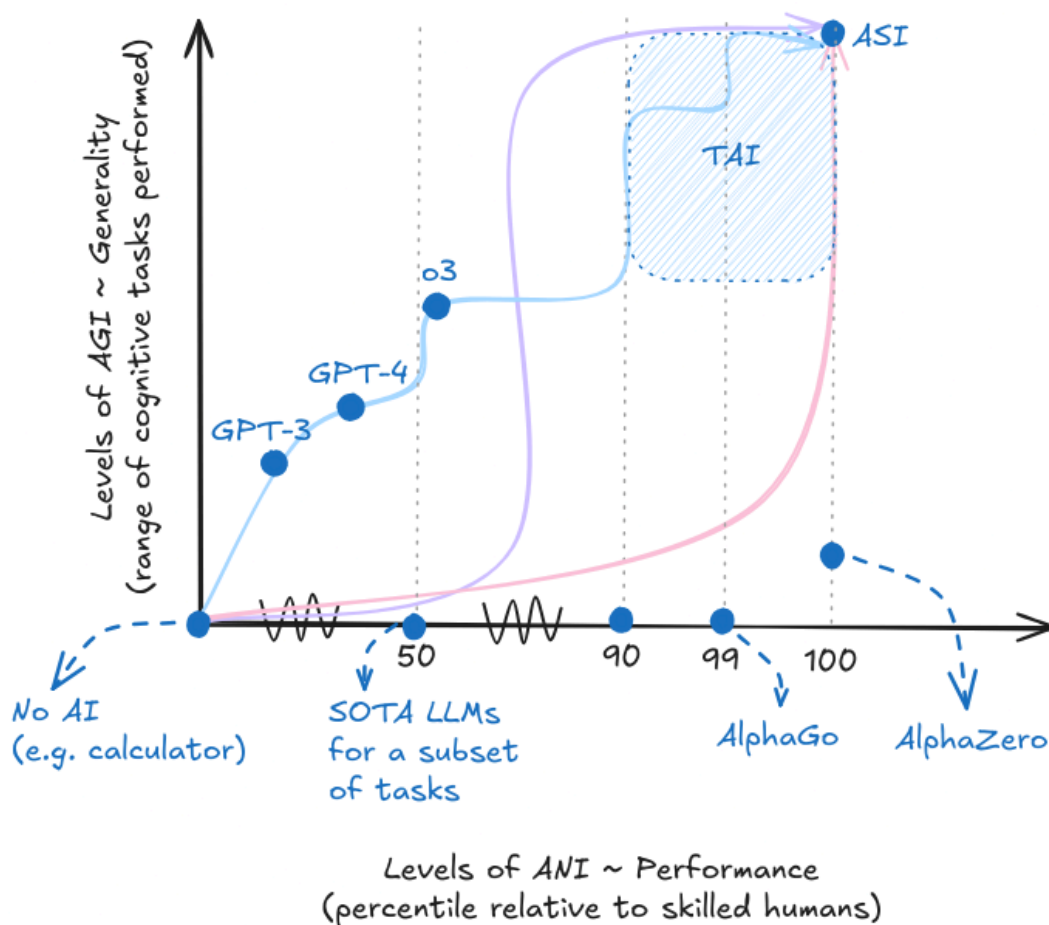
Figure 28: The two-dimensional view of capability \times generality. Different colored curves represent possible development paths to ASI. Every point on these paths corresponds to a different level of AGI capability.
