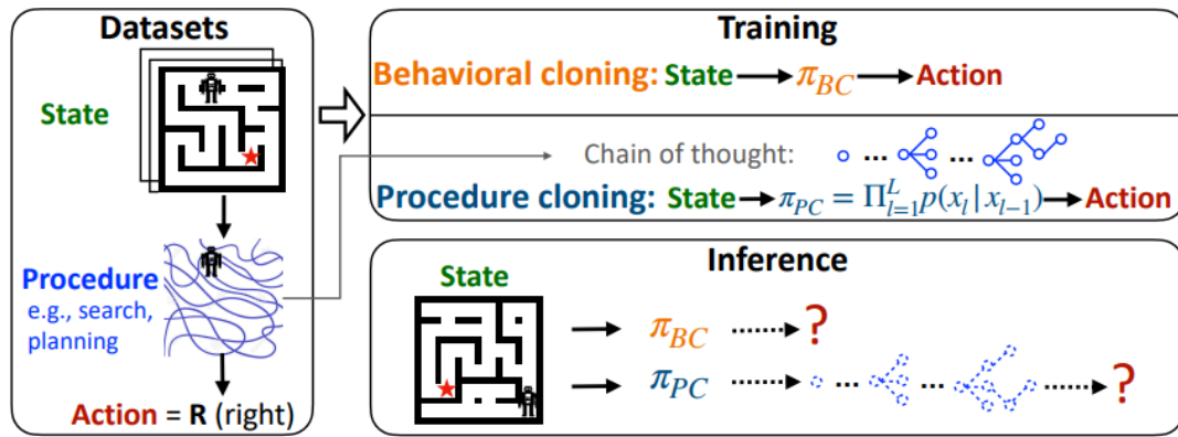
Figure 10: Visualization of the dataset collection, training, and inference of BC and PC on a maze navigation task. (Yang et. al; 2022)
