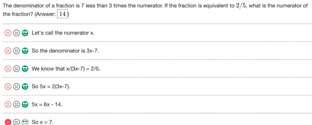
Figure 7: An example of process oversight feedback. The image is a screenshot of the interface used to collect feedback for each step in a solution. This shows the correct reasoning process being followed and reinforced, even if the ultimate answer is wrong. (Lightman et. al, 2023)
