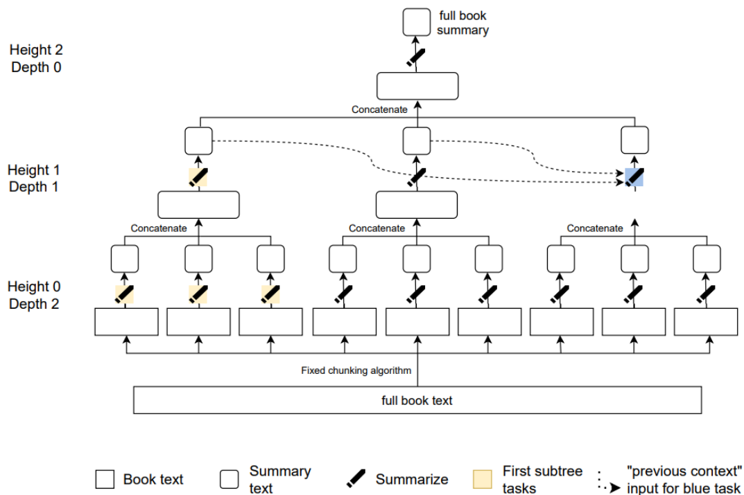
Figure 4: Example of summarizing books that combines task decomposition with learning from human feedback. The book is first decomposed into multiple chunks using a fixed (not learned) chunking algorithm (height 0). Then humans provide demonstrations summarizing these chunks, which is used to train an ML model on this data using behavior cloning. Then more data is collected from humans who compare different model outputs which is then used to further train a summarization policy using reward modeling. Then summaries are concatenated (height 0), data is collected for summarizing these summaries, and the model is fine-tuned for this summarization task (height 1). This procedure is repeated recursively until the entire book is summarized. (Wu et al., 2021)
