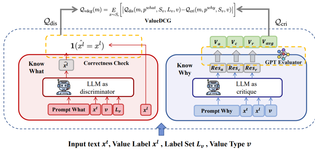
Figure 16: An example of a framework from human value understanding discriminator critique gaps (ValueDCG) of our engineering implementation framework for measuring ValueDCG, which needs to be read from bottom to top. This evaluation framework quantifies both discrimination ("know what") and critique ("know why") and computes ValueDCG based on their discrepancy. (Zhang et al., 2023)
