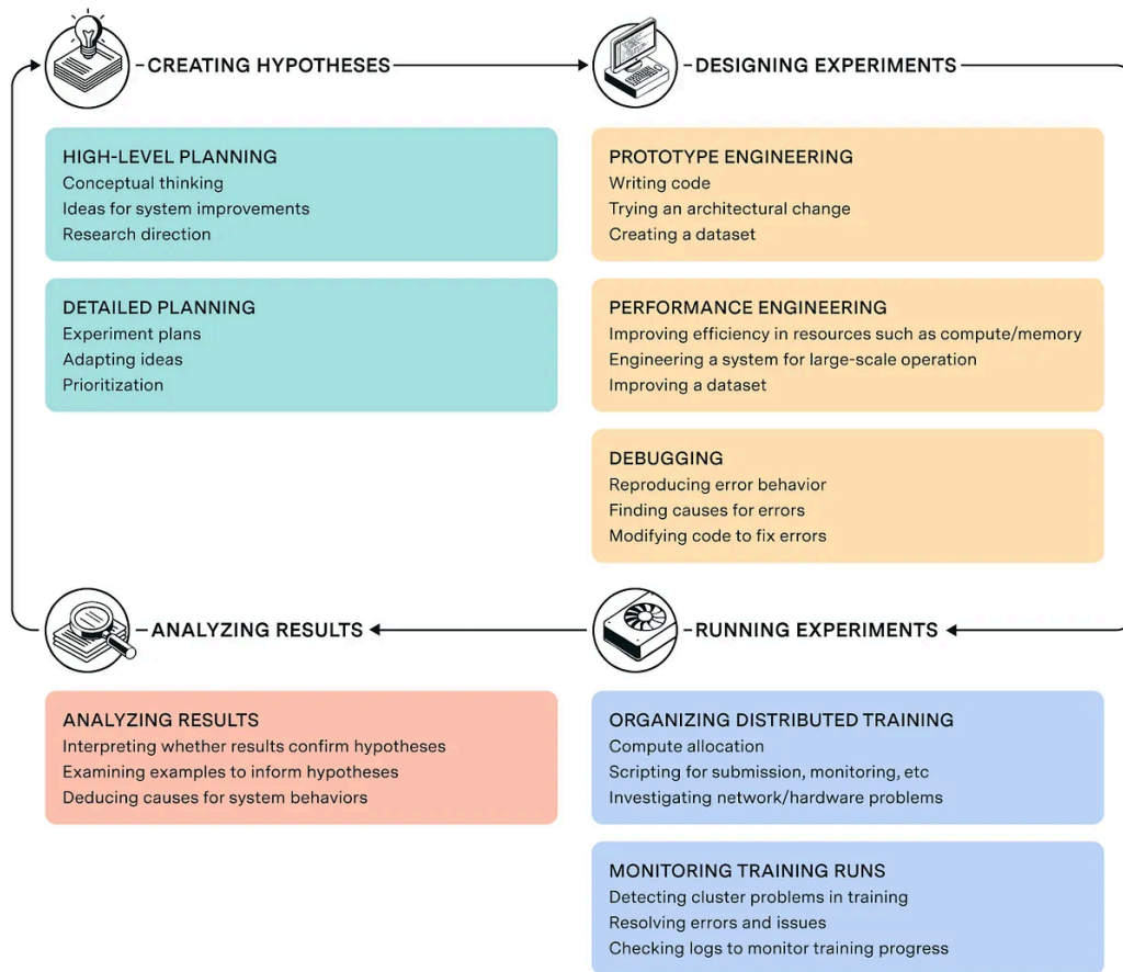
Figure 12: The AI Research and Development workflow. (Wiseman & McClements, 2025) How many of these tasks do you think can be amplified or even automated by having AI assistants?
