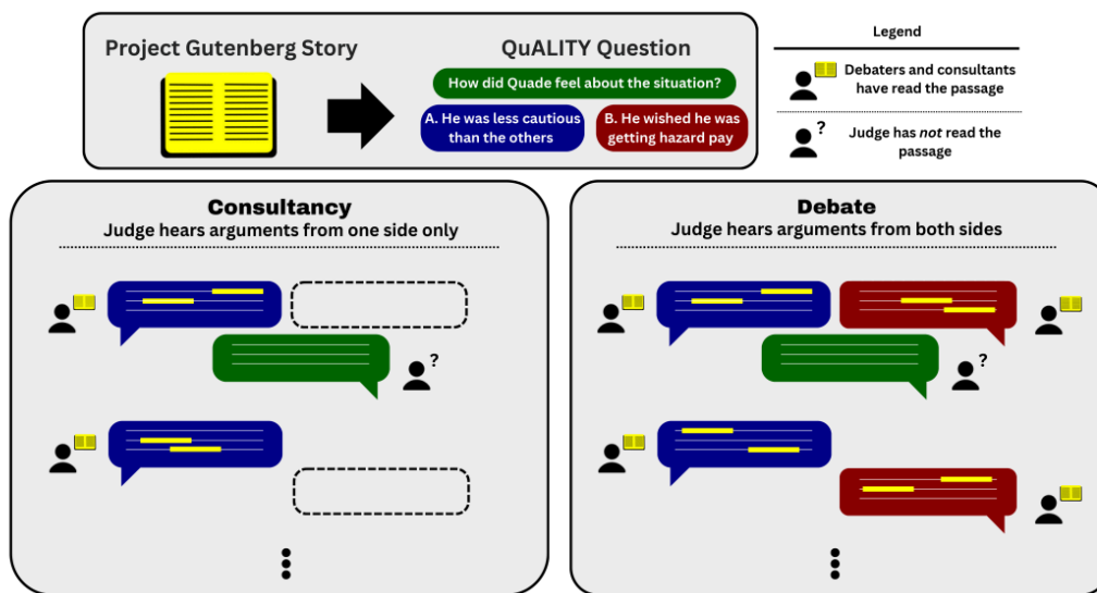
Figure 18: High level example of an experimental safety setup using AI debate. Reading comprehension
