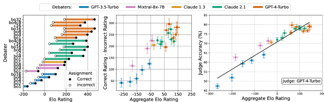
Figure 21: Stronger more persuasive debaters have been shown to result in better judge accuracy, whereas stronger consultants result in worse judge accuracy. ( Khan et al., 2024 )
