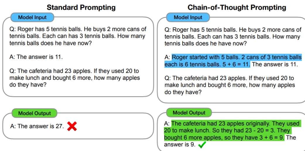
Figure 6: Prerequisite to overseeing the reasoning, is actually getting the model to output its reasoning. One common example is CoT prompting. CoT enables large language models to tackle complex arithmetic, commonsense, and symbolic reasoning tasks. (Wei et al., 2022) But it also allows us to oversee the “thought process” in addition to the final answer. (Lightman et. al, 2023)
