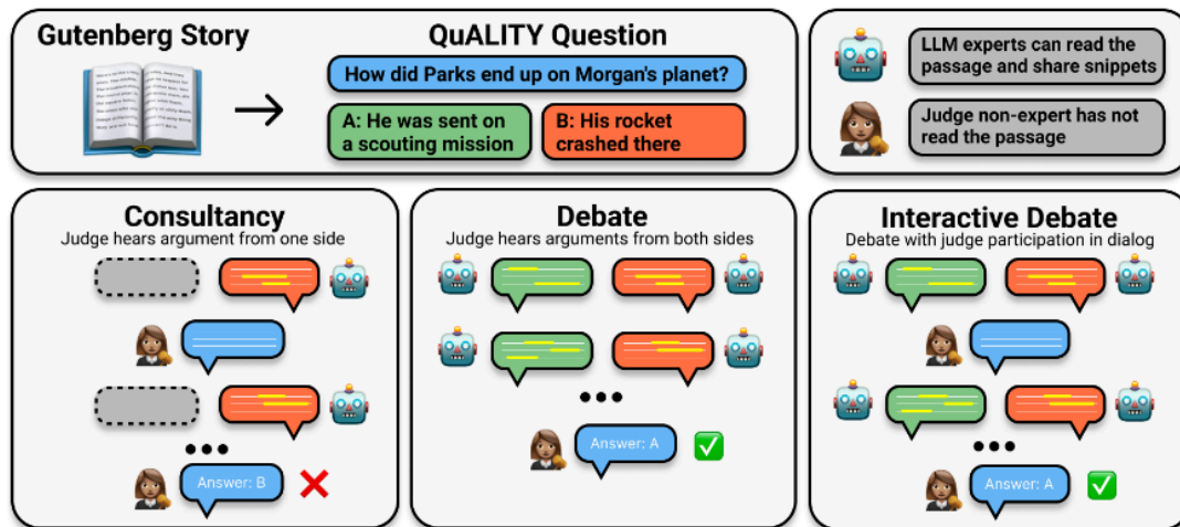
Figure 19: Expert models, who can access the underlying text from a project Gutenberg science-fiction story, argue for a specific answer to a comprehension question. Weaker (non-expert) judges, who cannot access the underlying text, evaluate the arguments and choose an answer. In debate, two experts simultaneously present arguments for a number of rounds. In interactive debate, the judge may ask clarifying questions after each round. In consultancy, a single expert argues for one of the two answers while the judge asks questions. (Khan et al., 2024)
