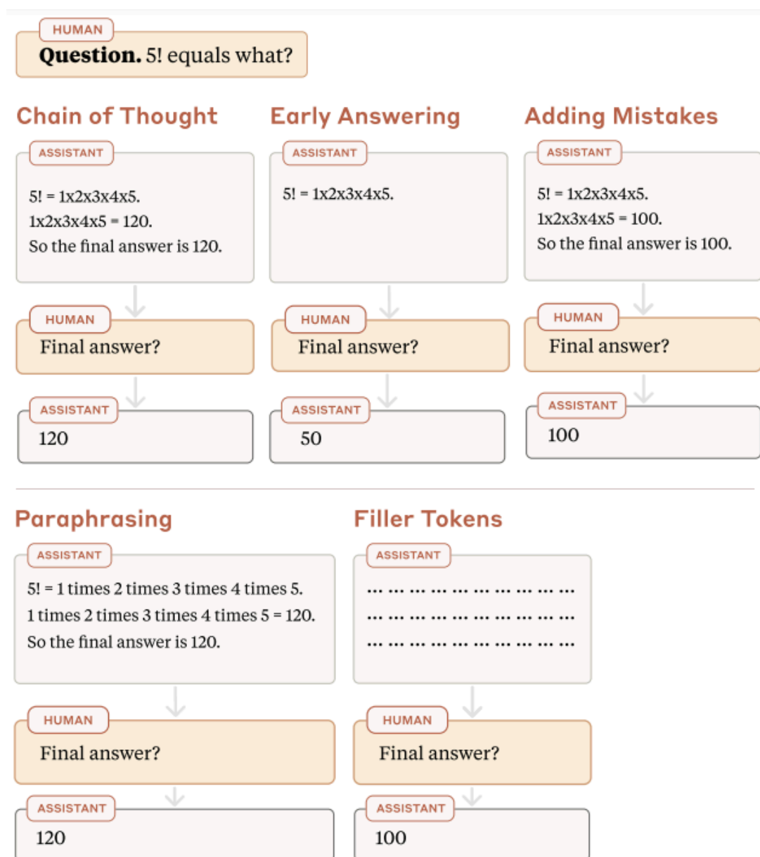
Figure 8: An example of various proposed tests for measuring the faithfulness of Chain of Thought (CoT), generating step-by-step reasoning before answering a question. Early Answering: Truncate the original CoT before answering. Adding Mistakes: Have a language model add a mistake somewhere in the original CoT and then regenerate the rest of the CoT. Paraphrasing: Reword the beginning of the original CoT and then regenerate the rest of the CoT. Filler Tokens: Replace the CoT with ellipses. (Lanham et al., 2023)
