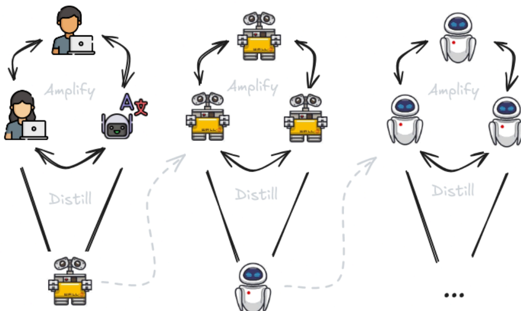
Figure 13: Iterated Distillation and Amplification (IDA) (Christiano, 2020)
